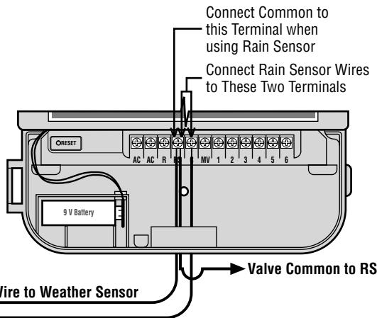
Sensor Wire to Common
