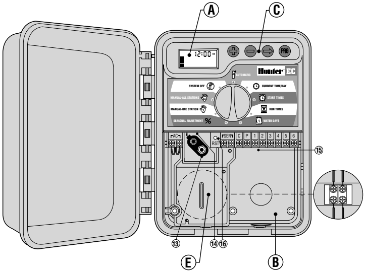
Outdoor Model (Internal Transformer Included)
